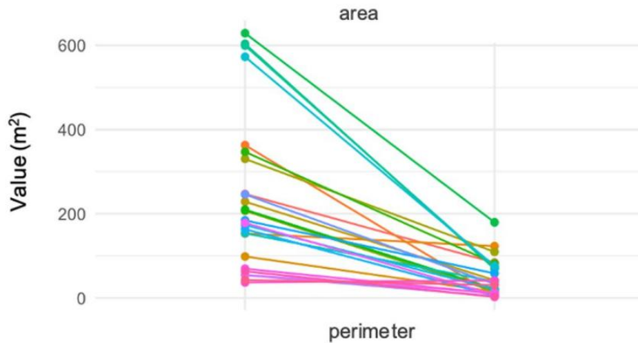
Figure 2: Our monitoring from last season showed a significant decrease in the size of anchor scars, where seagrass is infilling these areas of bare sand (Bibra, 2024). This has continued this season (see figure 3 below).
